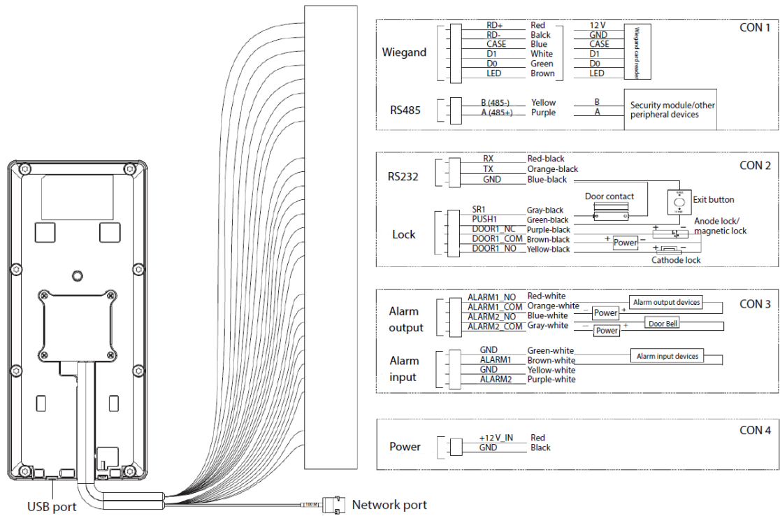
Figure 2-4 Wiring description
