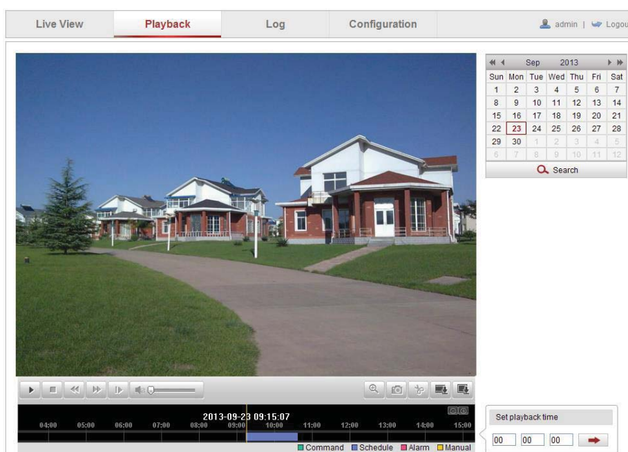
Figure 9-1 Interfejs odtwarzania
