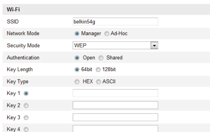
Figure 3-7 Tryb WEP
