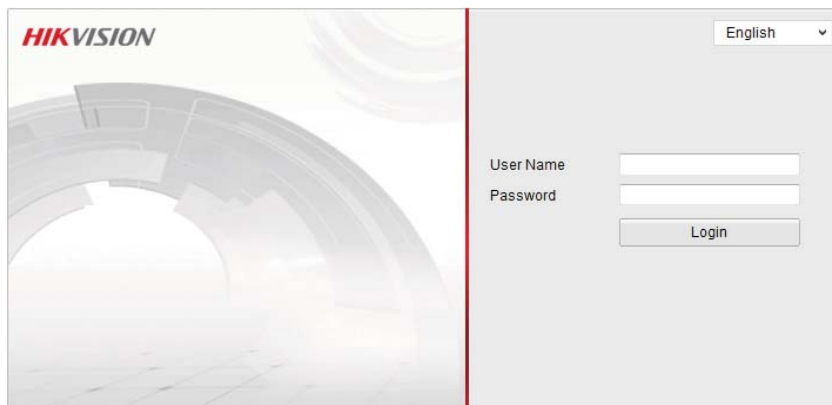
Figure 2-1 Interfejs logowania
