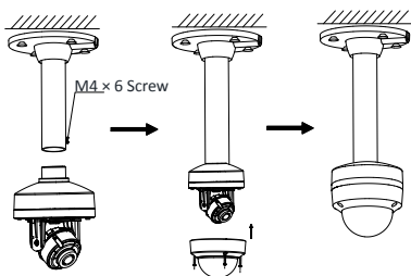
Figure 2-14 Finish Installation
