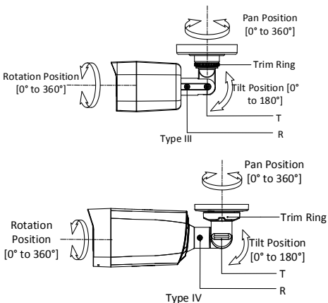
Figure 2-24 3-axis Adjustment
