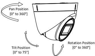
Figure 2-18 3-Axis Adjustment
