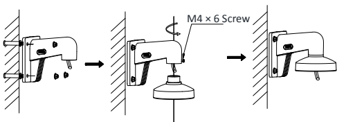
Figure 2-10 Install the Bracket
