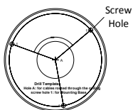
Figure 2-1 Drill Template
