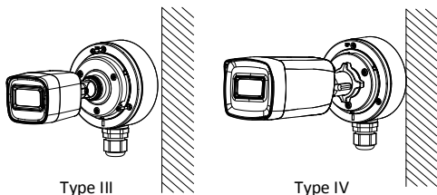
Figure 2-27 Combine the Junction Box Cover and Body
