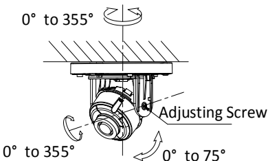
Figure 2-4 3-Axis Adjustment
