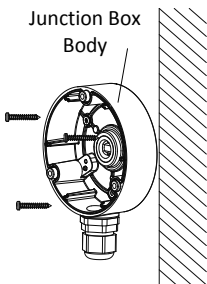
Figure 2-26 Secure the Junction Box on the Wall/Ceiling
