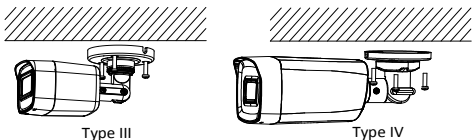
Figure 2-23 Fix the Camera to the Ceiling
