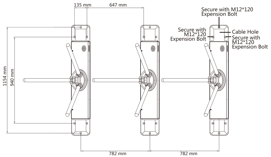
Figure 3-3 Installation Footprint
