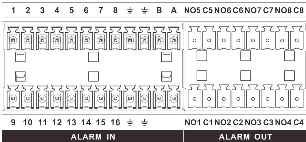
Figure 3-12 16/24-HDD series (2)
