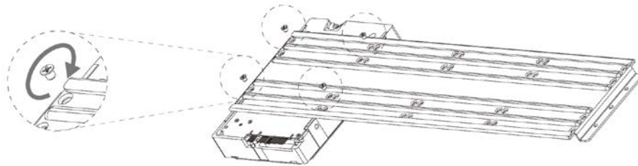
Figure 3-5 Install HDD (1)
