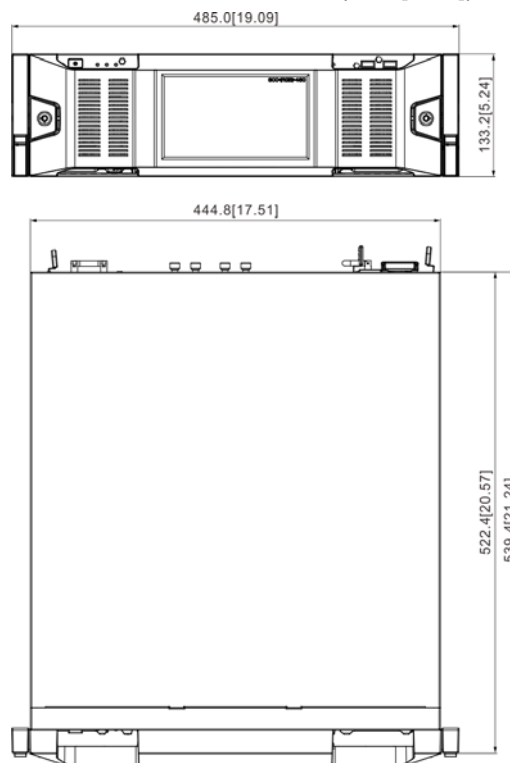
Figure 2-21 Dimensions with LCD (mm [inch])
