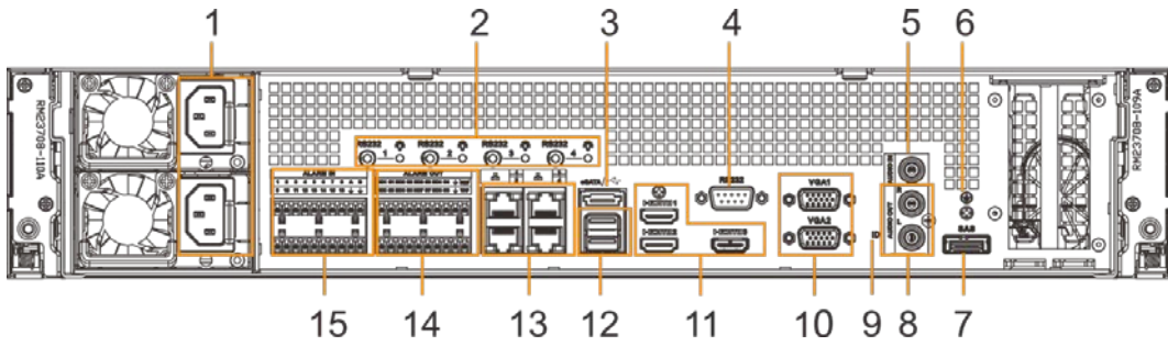
Figure 2-9 IVSS7012-M rear panel
