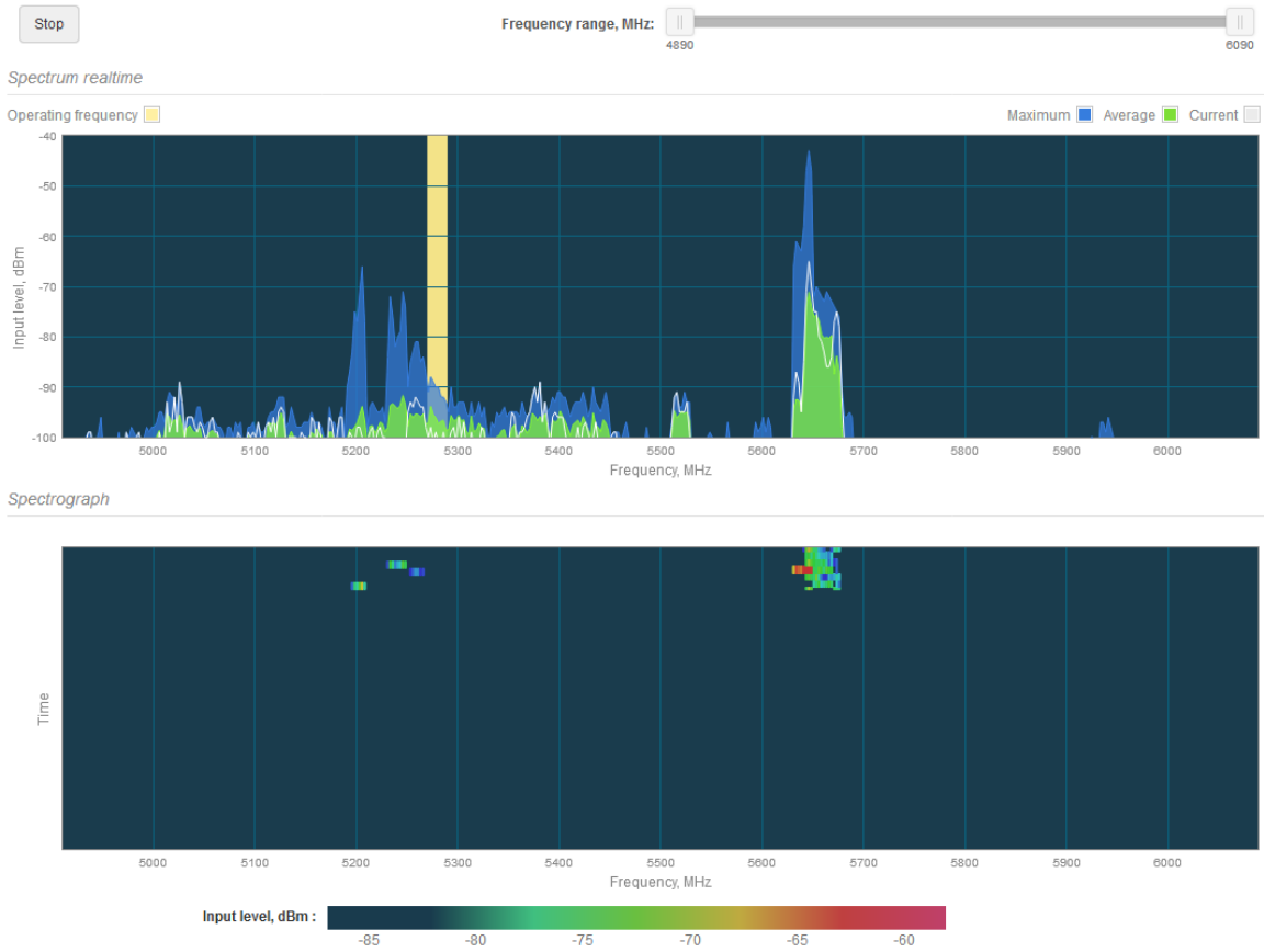
Figure 82 – Spectrum Analyzer Results
