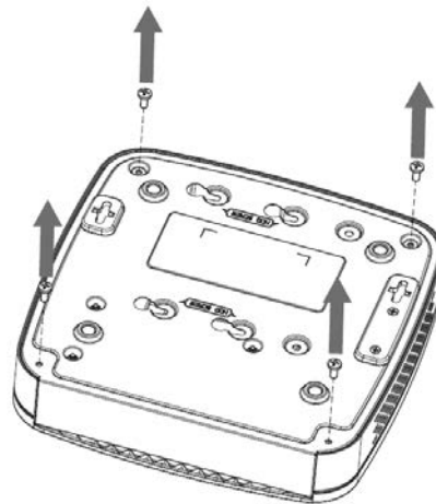
Figure 2-30 Remove screws
