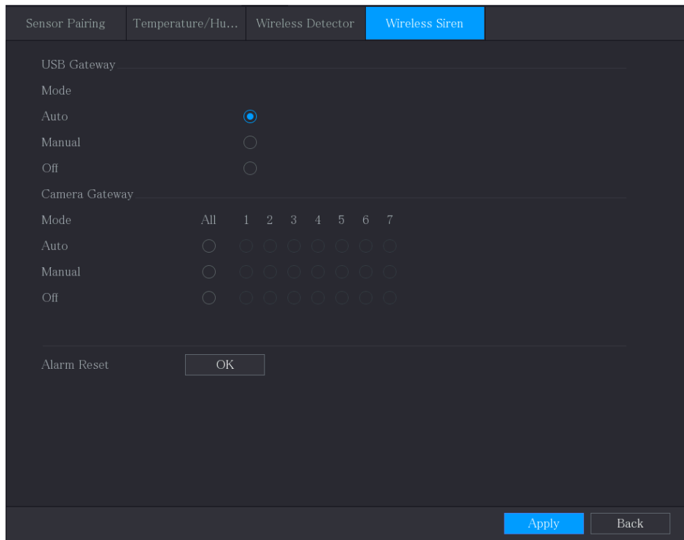
Figure 5-269 Wireless siren
