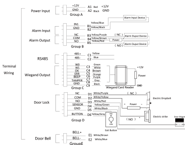
Figure 4-2 External Device Wiring
